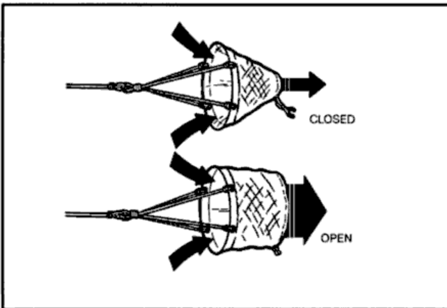
Figure 16-5. Sea anchor.
